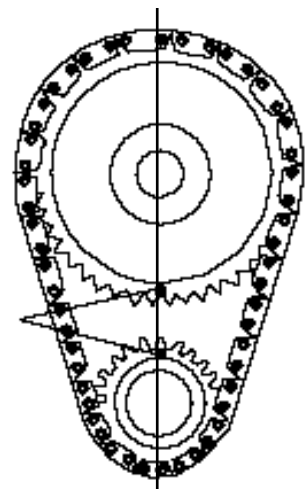
Figure 2- Timing Chain Sprocket Alignment
